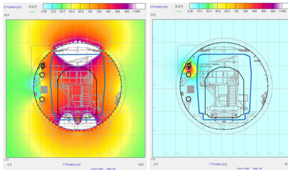
Catenary fault
