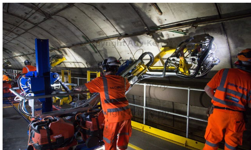
Figure 9: Drilling module
